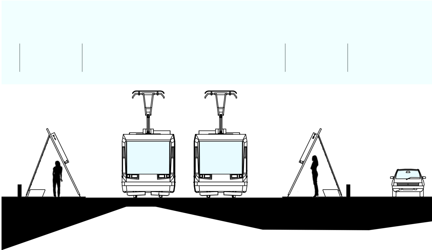
SECTION 1:100
